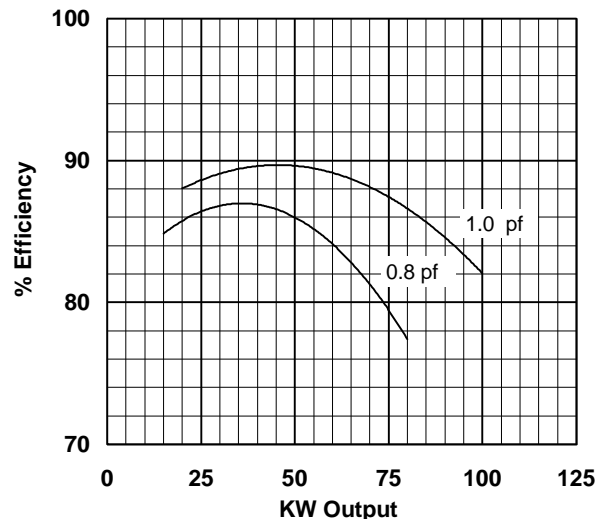
TYPICAL GENERATOR EFFICIENCY
