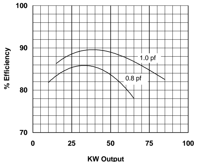
TYPICAL GENERATOR EFFICIENCY
