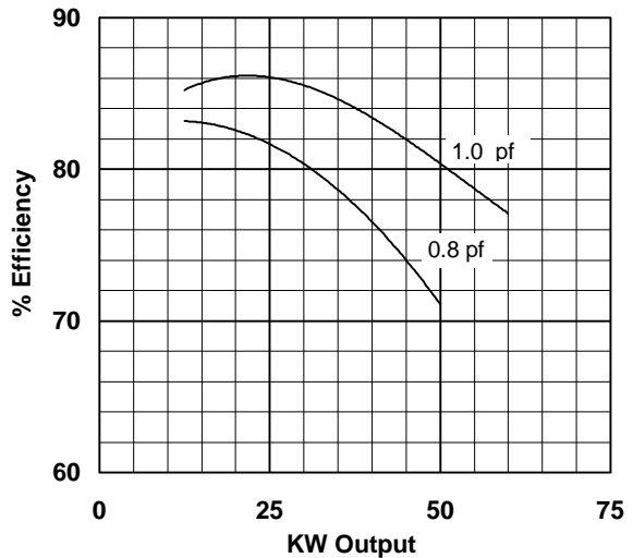
TYPICAL GENERATOR EFFICIENCY
