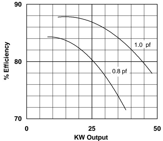
TYPICAL GENERATOR EFFICIENCY
